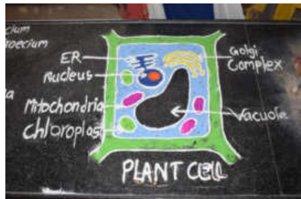
Plant Cell
